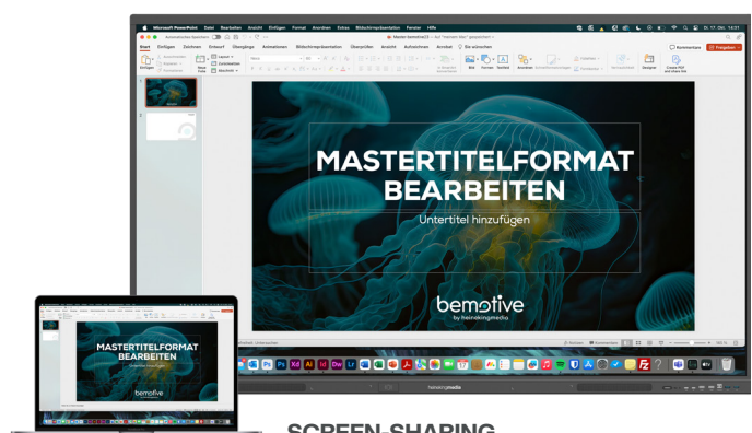
SCREEN-SHARING
